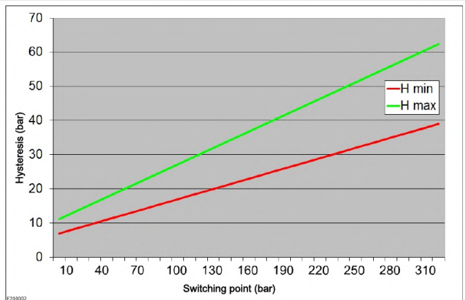
Piston version
